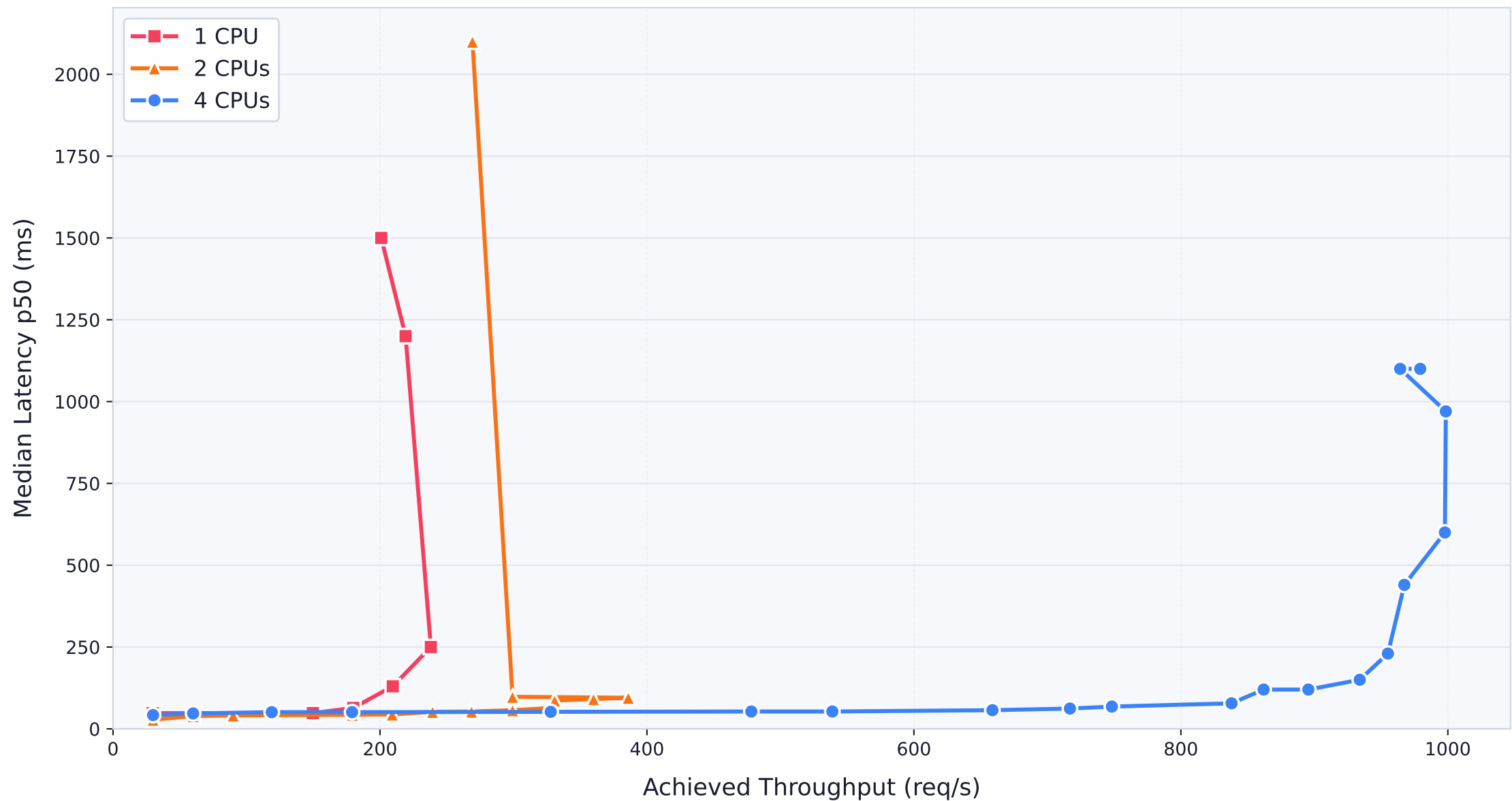
Context 2 — Latency vs Throughput (sorted by latency)
