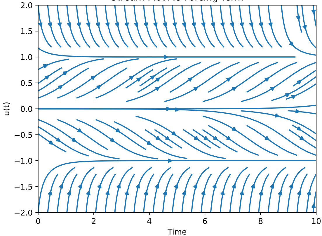
Stream Plot AC Forcing Term
