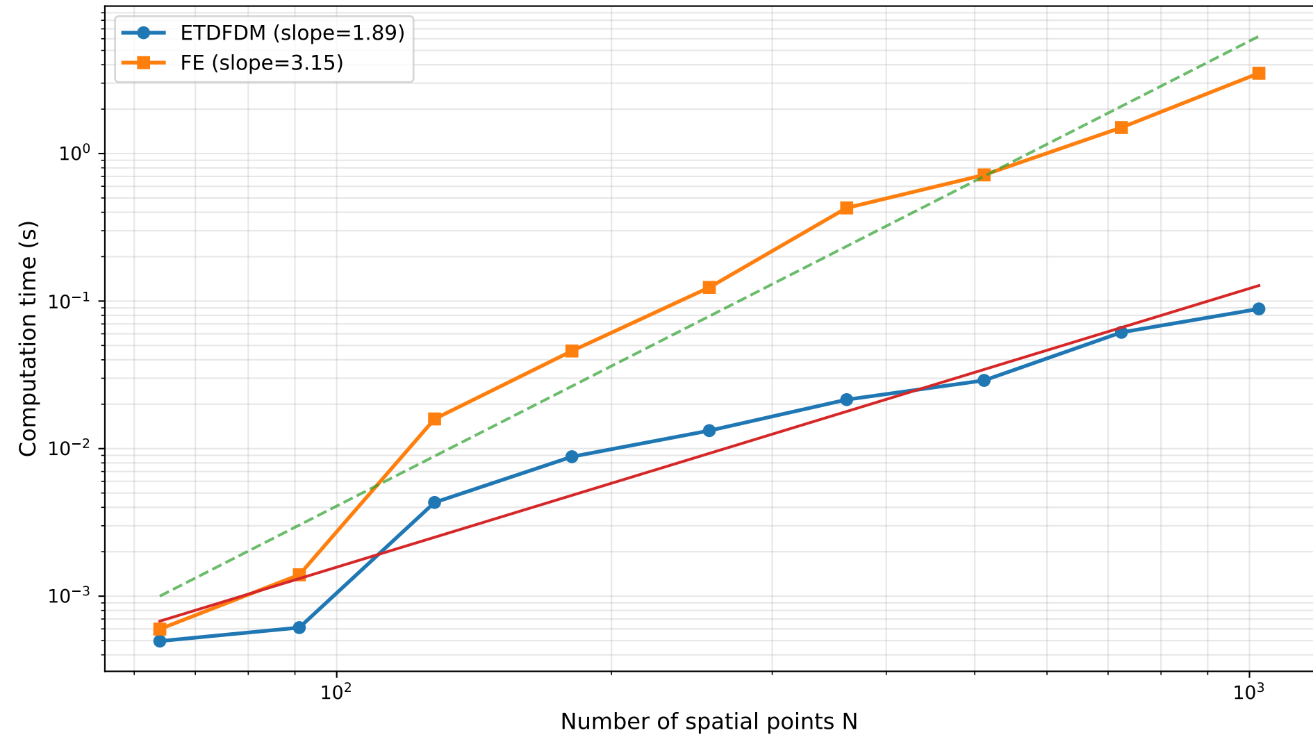
Runtime Scaling: ETDFDM vs Forward Euler
