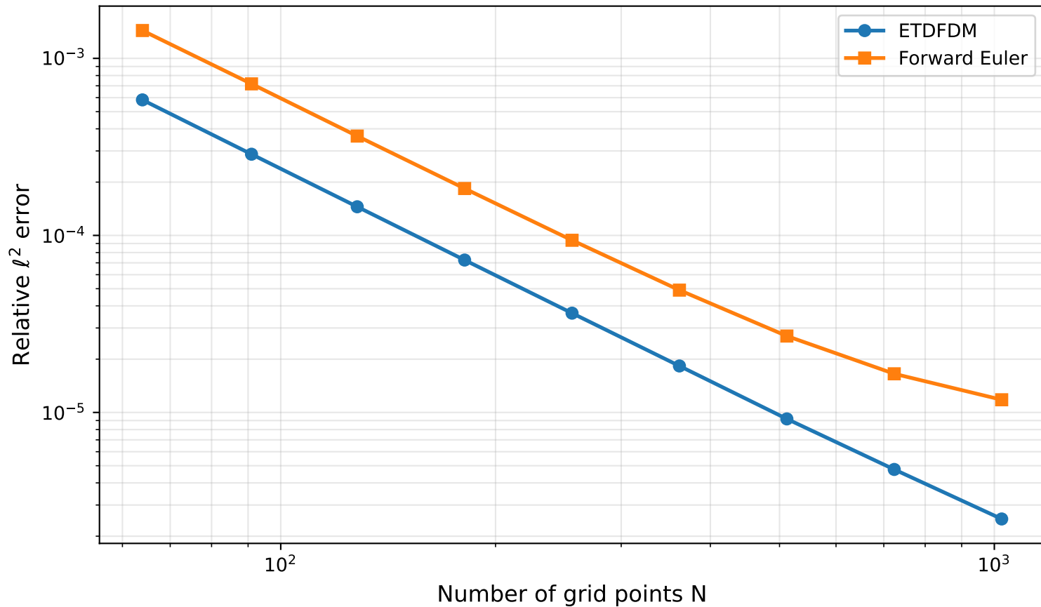
Error vs Number of Grid Points
