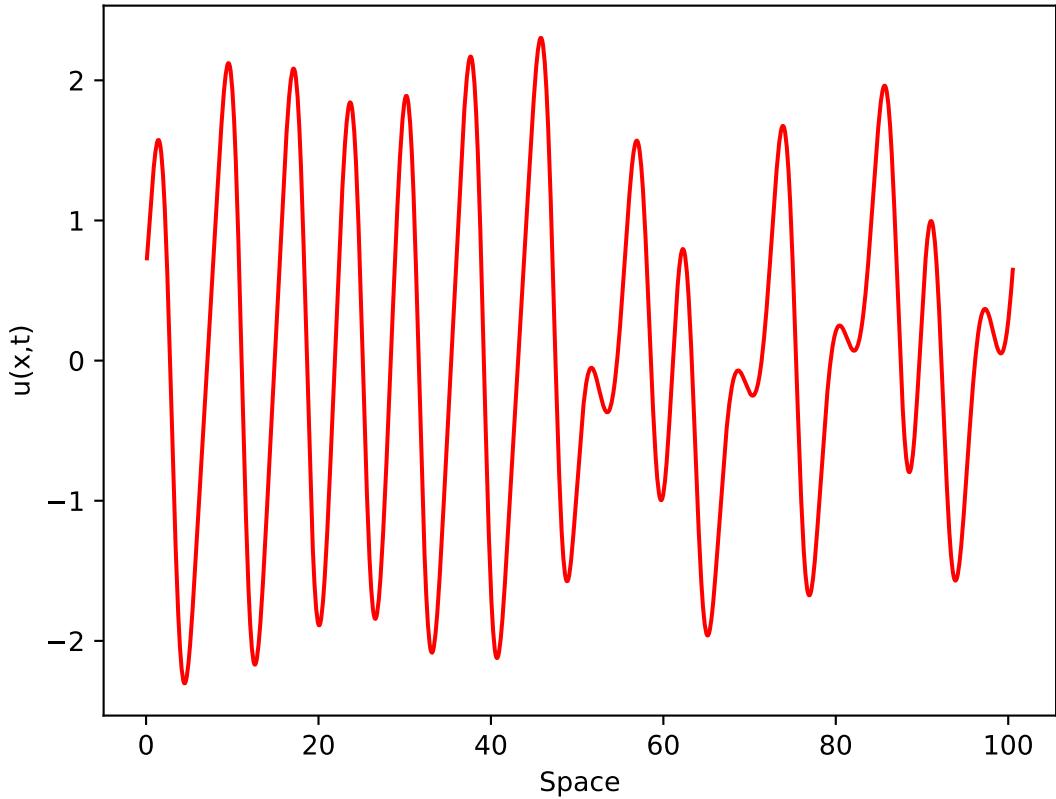
Kuramoto-Sivashinsky Transient Solution
