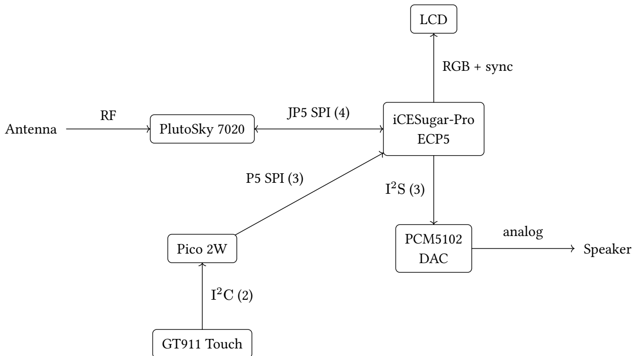
Figure 6: Physical wiring of the four boards. The label on each link gives the bus and its wire count; exact pin assignments are in the connection table.
