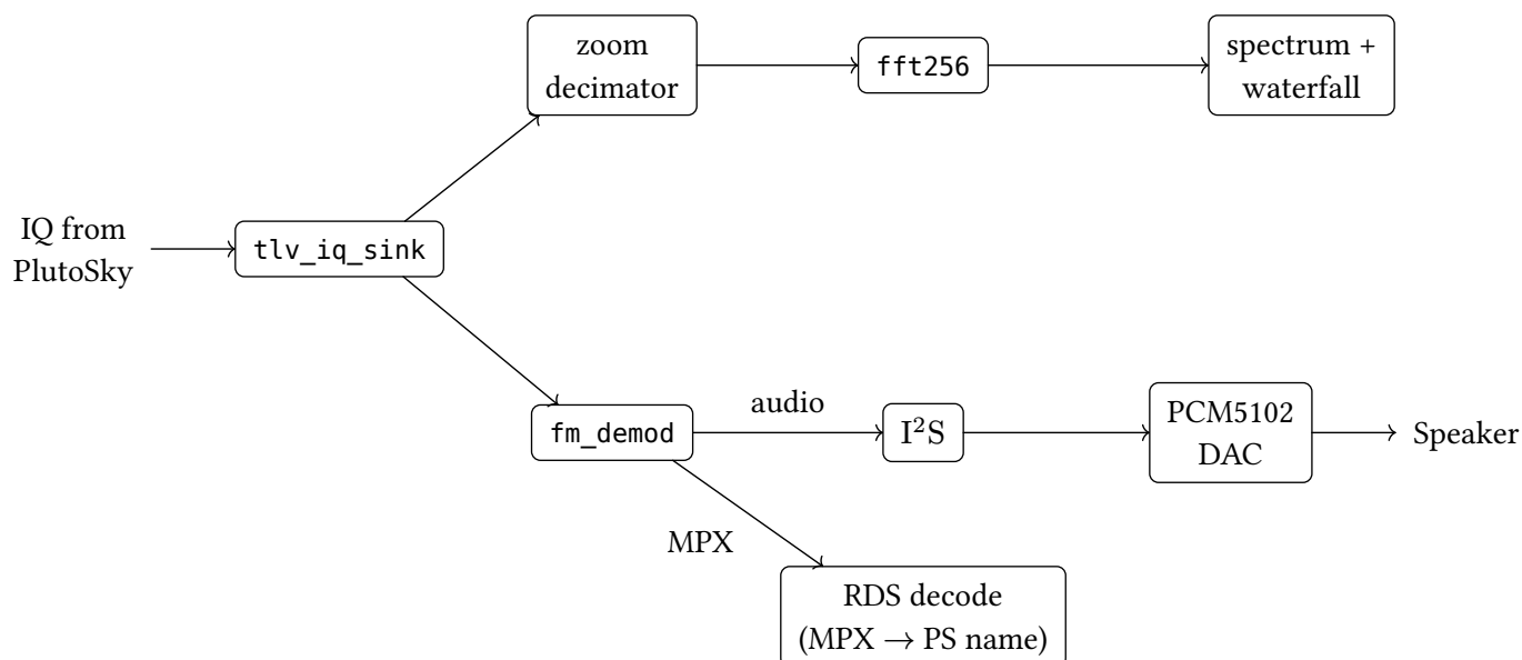
Figure 4: The FM signal-processing chain inside the ECP5. One IQ stream splits three ways: an FFT branch that feeds the spectrum and waterfall, an audio branch through the FM demodulator to the DAC, and an RDS branch that recovers the station name from the FM multiplex. The spectrum and waterfall outputs are written to SDRAM by the compositor in the display pipeline.
