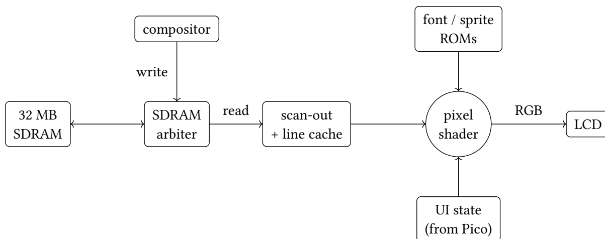
Figure 5: The display pipeline. The waterfall and image regions live in SDRAM; the compositor writes them and a scan-out reader pulls one line ahead into an on-chip cache. The pixel shader composes the final image on the fly, overlaying live UI elements from font and sprite ROMs and the current UI state on top of the SDRAM-backed line, and emits one RGB pixel per clock to the LCD.
