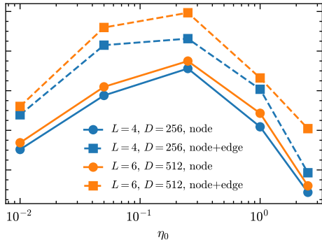
CAPEN-Llama
