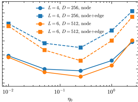
CAPEN-Llama
