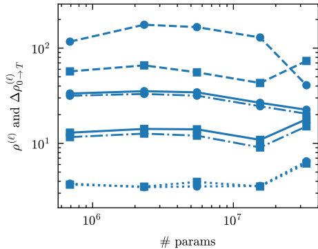
After T=100 Adam steps
