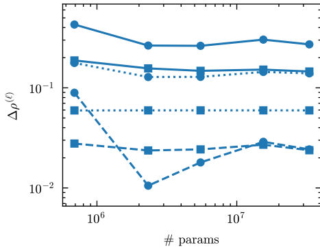
After 1 Adam step
