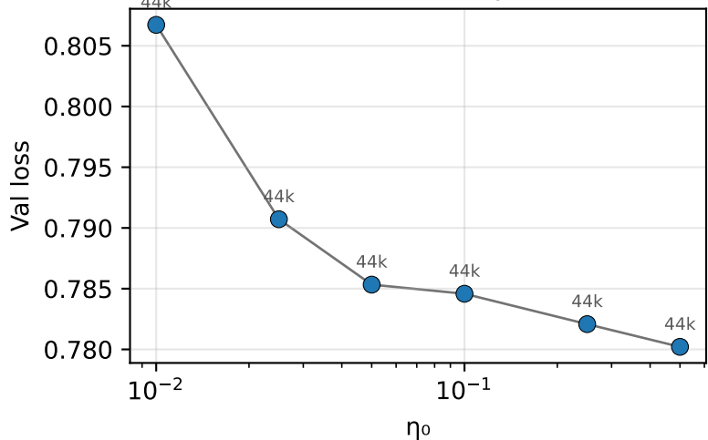
Val loss vs \eta_0
