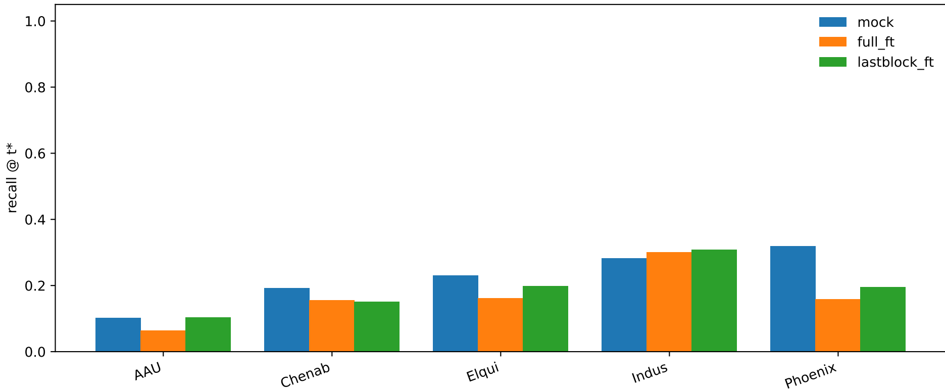
Holdout recovery: mock vs fine-tunes
