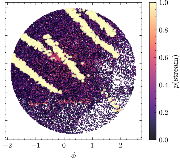
predicted AUROC=0.997
