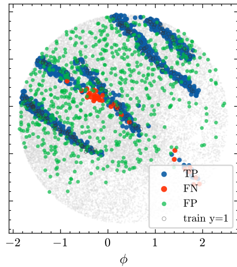
discovery @ p_i=1.00 P=0.57 R=0.96 TP=876 FP=651 FN=32
