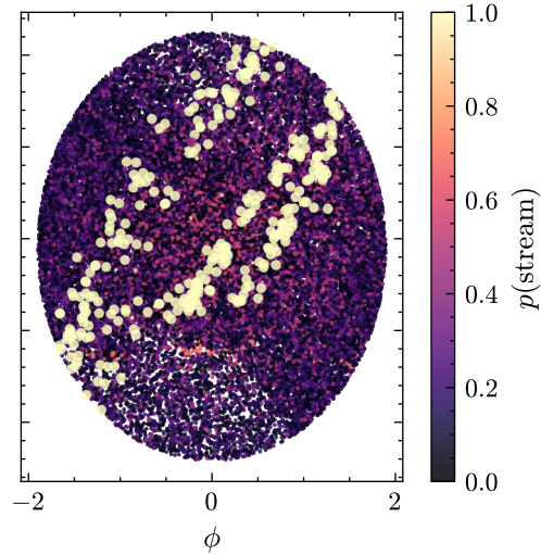
predicted AUROC=0.998
