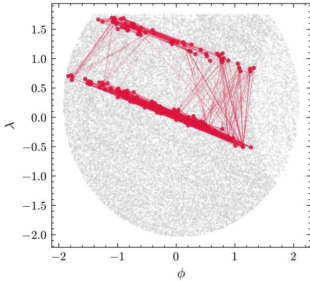
MOCK'1863 truth y+=181
