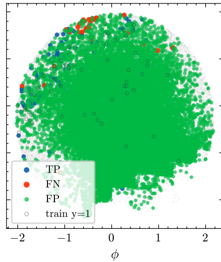
discovery @ p_i=0.5 TP=160 FP=32198 FN=58
