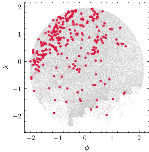
MOCK'2041 truth y+=283
