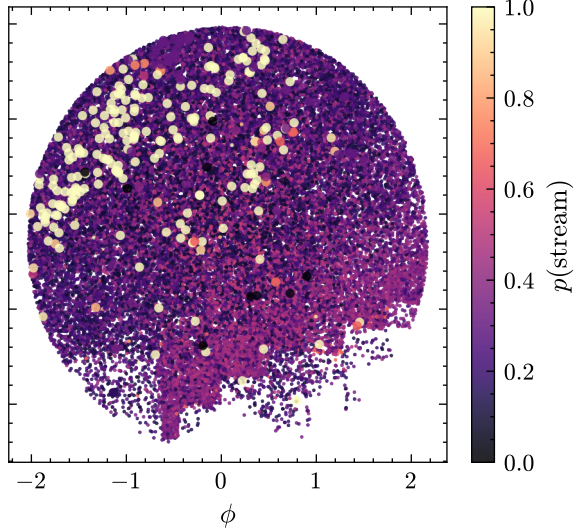
predicted AUROC=0.860 P=0.00 R=0.73
