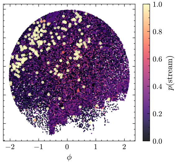
predicted AUROC=0.893
