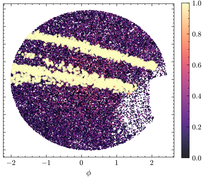
predicted AUROC=0.998
