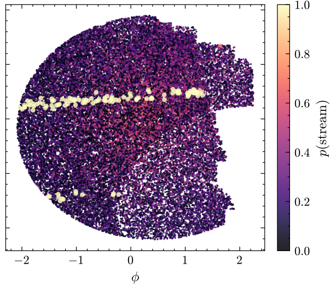
predicted AUROC=0.995
