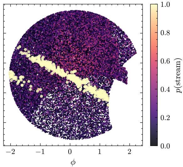
predicted AUROC=0.997
