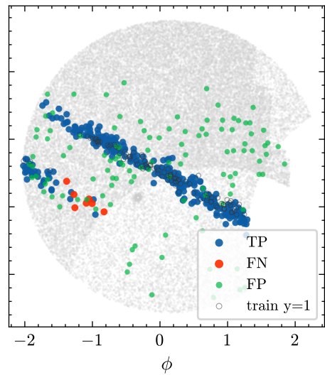
discovery @ p_i=1.00 P=0.73 R=0.98 TP=311 FP=116 FN=7
