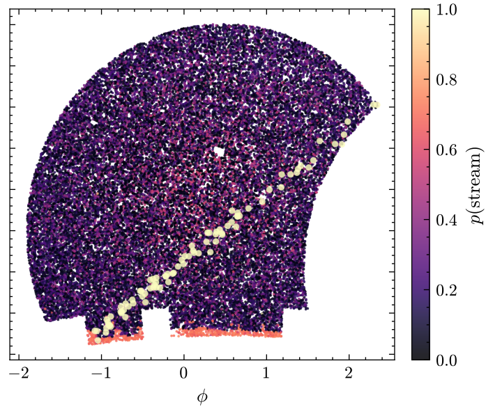
predicted AUROC=0.999
