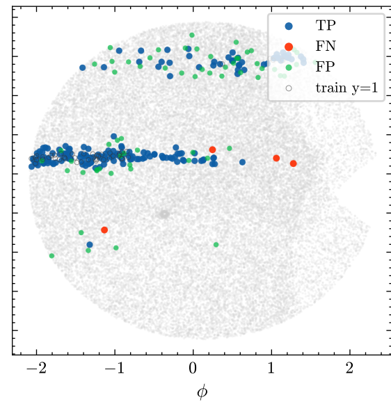
discovery @ p_i=1.00 P=0.74 R=0.98 TP=175 FP=63 FN=4
