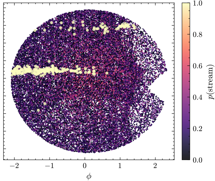
predicted AUROC=0.999
