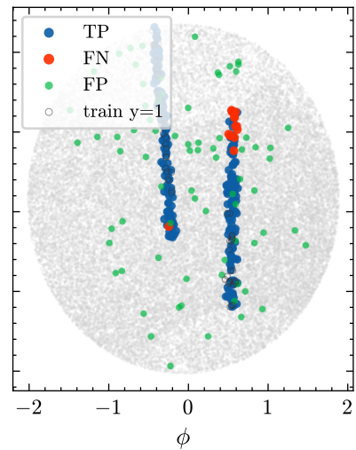
discovery @ p_i=1.00 P=0.76 R=0.94 TP=240 FP=75 FN=14
