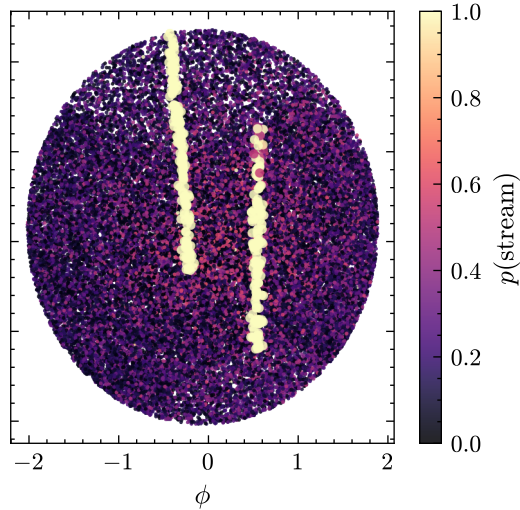
predicted AUROC=0.997
