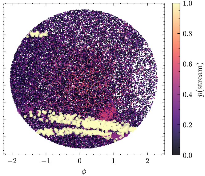
predicted AUROC=0.956
