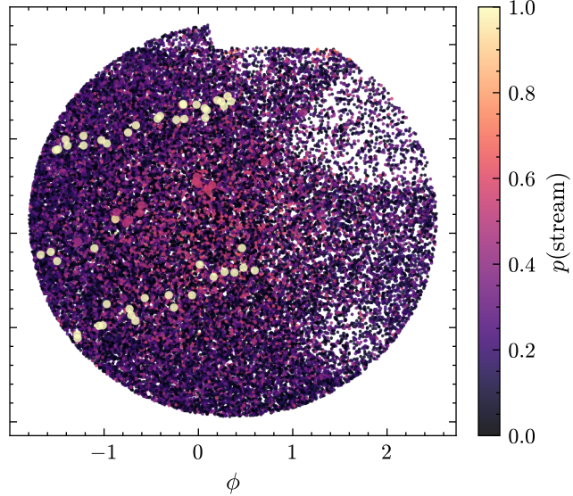
predicted AUROC=0.978
