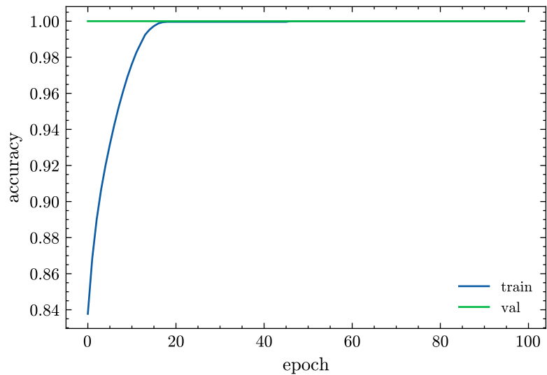
Supervised-pool accuracy
