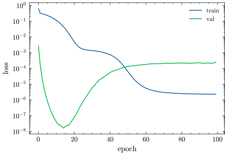
CE loss
