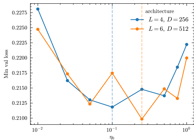
Min val loss vs \eta_0
