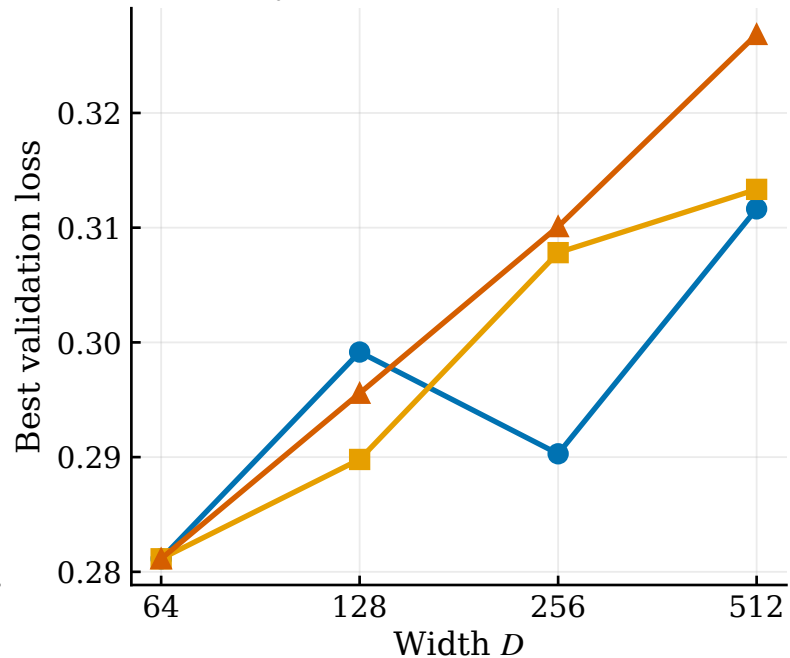
Width transfer of best-over-run loss \cdot \eta_0^* = 0.05
