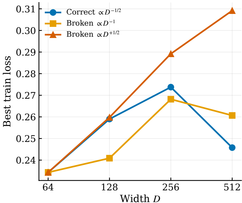
Width transfer of best-over-run loss \cdot \eta_0^* = 0.05
