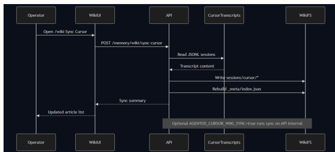
Wiki sync sequence
