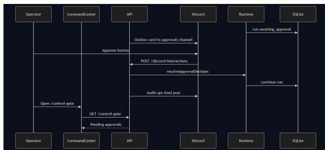
Approval gate sequence
