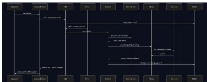
Mission run sequence
