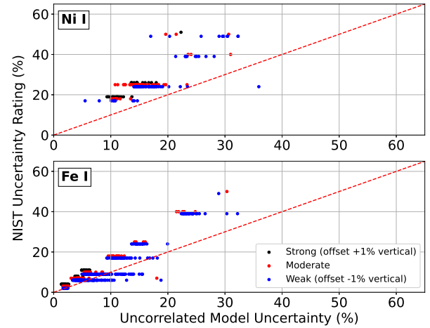
Figure 3. (Top) Model uncertainties for the fluorescence spectrum of Ni I, calculated as the standard deviation of fluorescence efficiencies as a percentage of the value with the default transition rate following 10^5 iterations within the limits of \pm the Atomic Spectra Database (ASD) accuracy (see Table 1 of the published article) versus the ASD accuracy rating for 163 selected nickel transitions with model uncertainties <100\% . Axis limits were restricted to enhance the visibility of the majority ( >99\% ) of lines within this criterion. Strong and weak lines are offset \pm 1\% vertically with respect to moderate lines for visibility; for definitions of line classifications, see text in the published article. (Bottom) Fe I model uncertainties versus ASD accuracy ratings for 645 transitions with uncertainties lower than 100\% .
