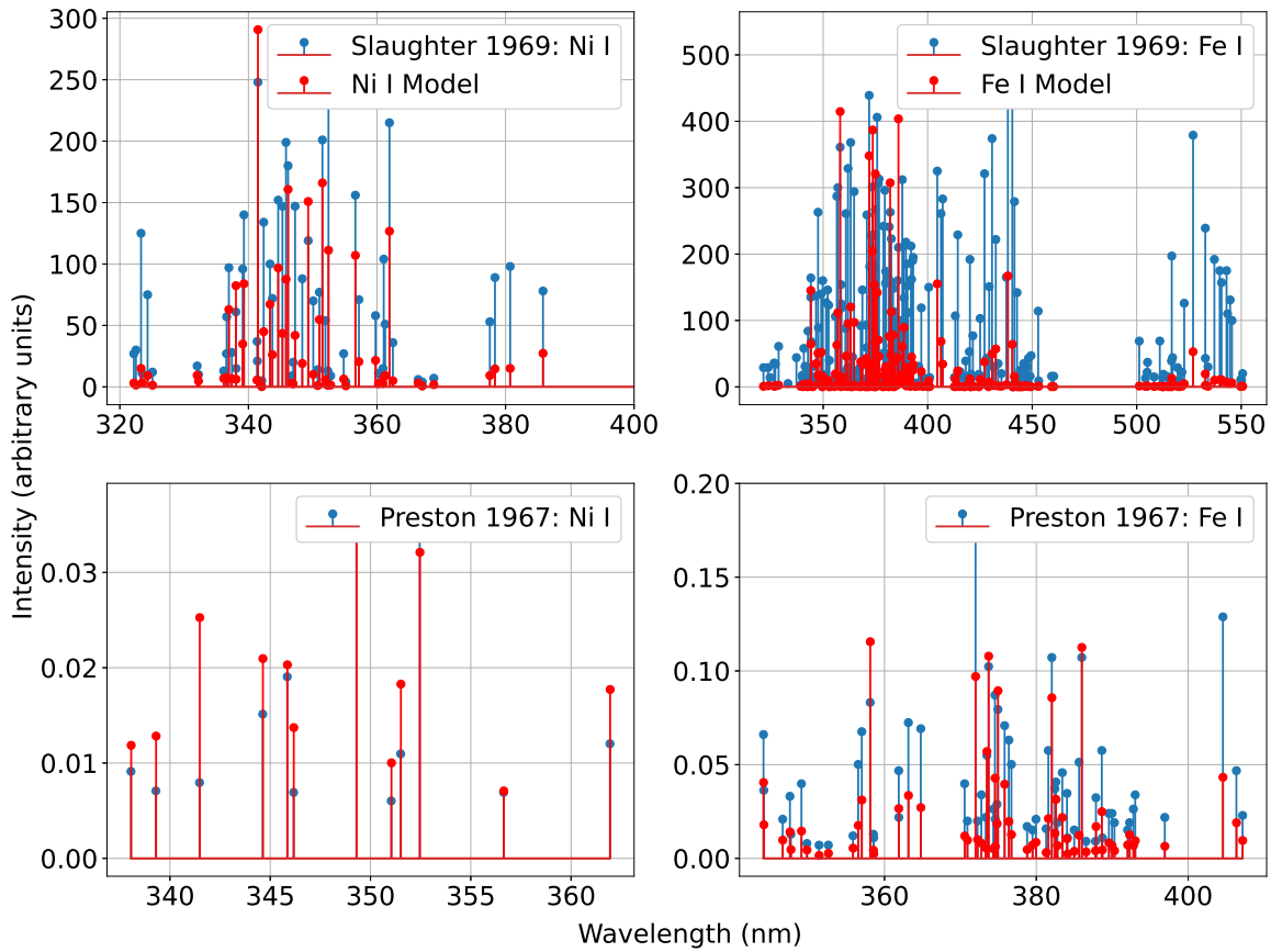
Figure 4. Comparison of Ni I (left) and Fe I fluorescence models (in photon units) to the observed intensities in comet C/1965 S1 (Ikeya-Seki) as reported in C. D. Slaughter (1969) (top) and G. W. Preston (1967) (bottom). The model spectra are scaled via a linear fit of all present lines. Doppler line profiles were assumed for equilibrium temperatures derived from the heliocentric distances: 1081 K (C. D. Slaughter 1969) and 743 K (G. W. Preston 1967).
