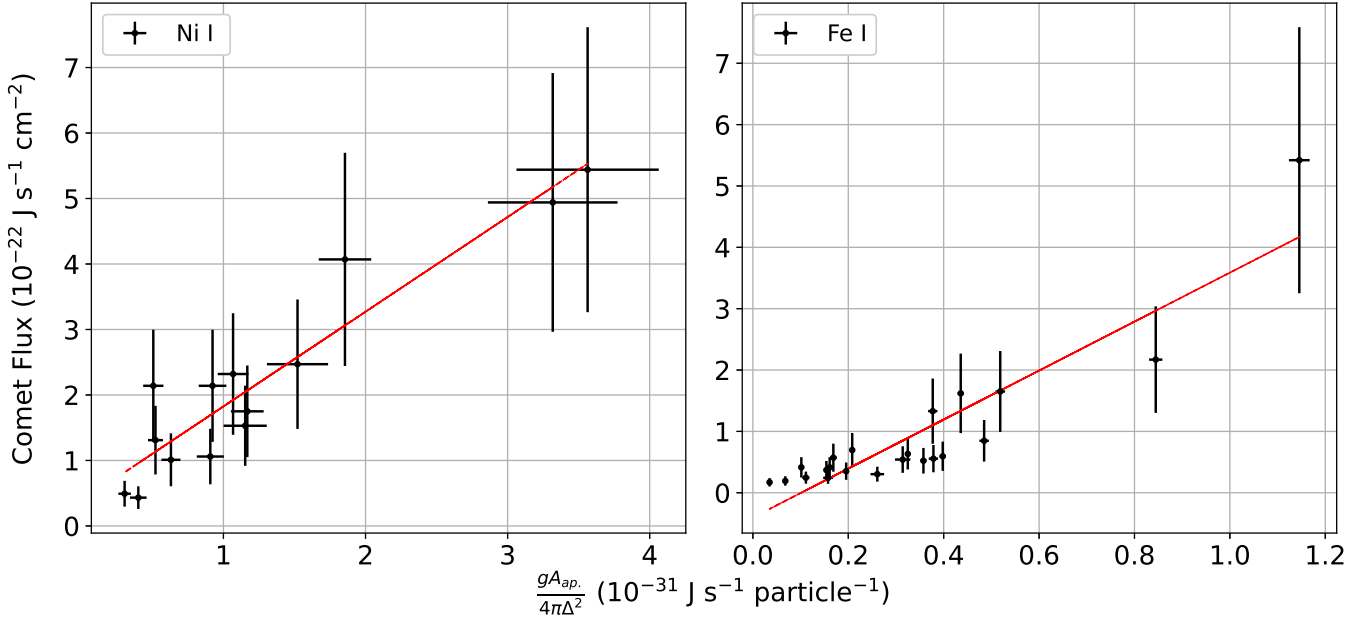
Figure 7. Comparison of fluorescence efficiencies (with geometric factors) and observed fluxes of Ni I (left) and Fe I (right). Model error bars are taken from the Monte Carlo iterations of the fluorescence model within the stated Einstein A coefficient uncertainty. An absolute error of \pm 40\% was assumed for the observed fluxes (R. Meier et al. 1998). The linear fit used to compute the column densities is shown in red for each atom.
