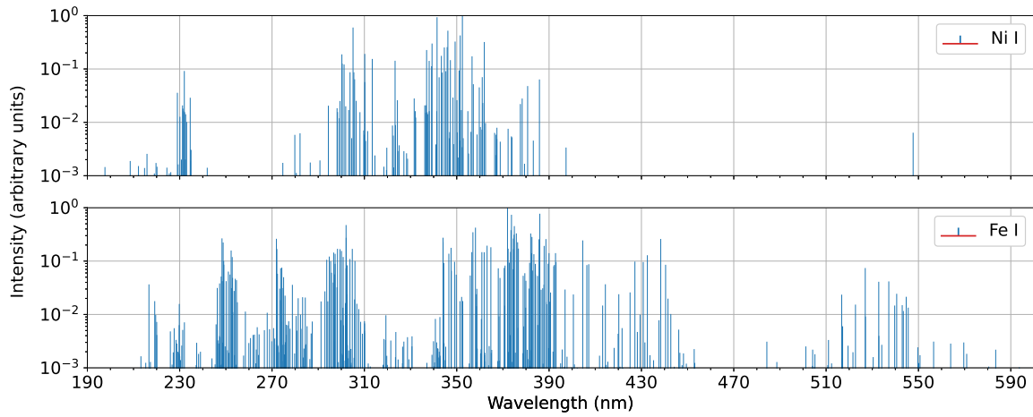
Figure 1. Fluorescence spectra stick plots on a logarithmic intensity scale with the strongest lines normalized to 1 for Ni I (top) and Fe I (bottom) spanning 190–600 nm. Fluorescence efficiencies were calculated for the observing conditions of C/1996 B2 (Hyakutake), v_h = -36.7 \text{ km s}^{-1} and r_h = 1.02 \text{ au} .
