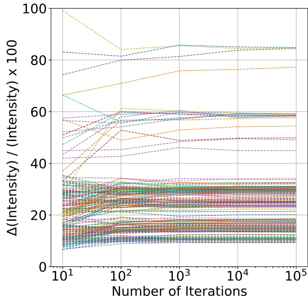
Figure 2. Ratio of fluorescence efficiency standard deviation to fluorescence efficiency (in percentage) for Ni I lines spanning 300–500 nm as a function of iteration number, generated for 10 , 10^2 , 10^3 , 10^4 , and 10^5 iterations. Each colored line shows the convergence of an individual transition.
