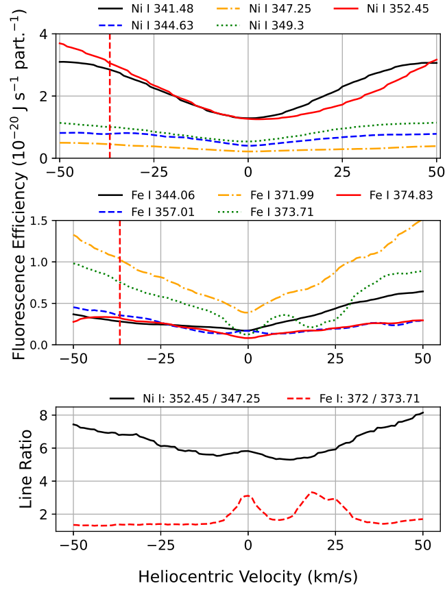
Figure 10. Sensitivity of our modeled fluorescence efficiencies for some representative Ni I lines (top) and Fe I lines (middle) to heliocentric velocity, and (bottom) example velocity-sensitive line ratios for Ni I (black) and Fe I (red). Efficiencies were calculated for a heliocentric distance of 1 au. The heliocentric velocity of Hyakutake ( -36.7 \text{ km s}^{-1} ) is shown as a vertical dashed line.
