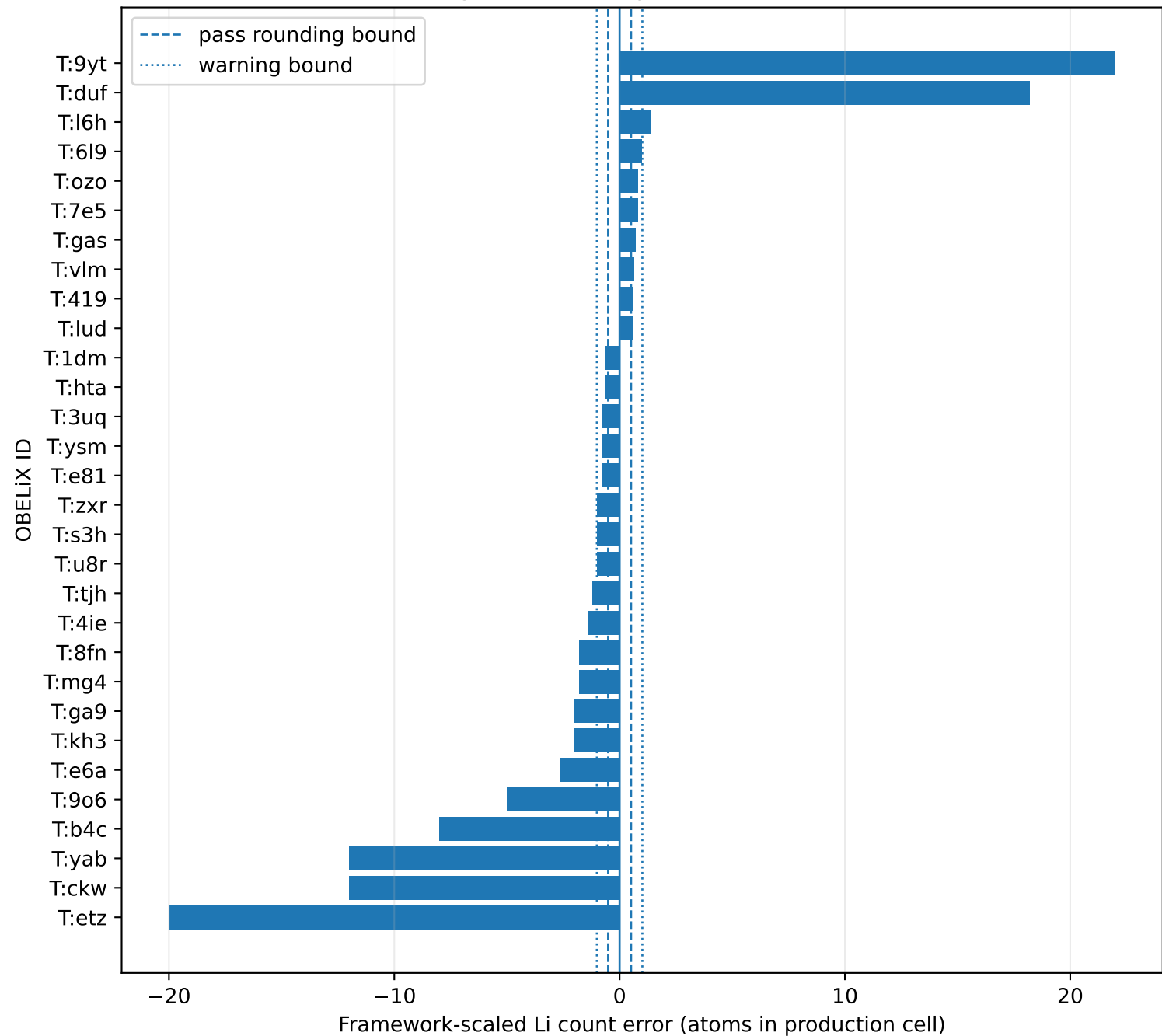
Largest Li/vacancy count deviations
