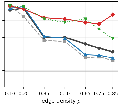
qwen3-1.7b-think
