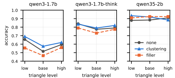
Figure 6: Rewiring: node_degree accuracy by triangle level (200 graphs per level; degree sequence and prompt length fixed; mean clustering 0.01, 0.31, 0.73).
