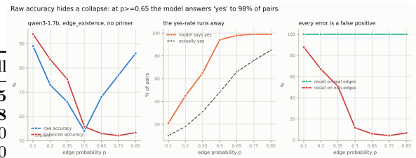
Figure 3: edge_existence under none, qwen3-1.7b. Accuracy falls to 54% at p=.50 and then rises again to 86% at p=.85 , which reads as a recovery. Balanced accuracy over the same responses does not recover: it reaches chance at p=.65 and stays there, because the model answers “yes” to 98–99% of pairs while 66–85% of them really are edges.
