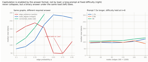
Figure 4: The response-length collapse on edge_existence and two controls on it. (a) median new tokens by density under none for three tasks answered about the same graphs: only the task with a two-valued answer collapses, while the tasks that must enumerate keep generating, so the trigger is not the graph. (b) median new tokens against n at fixed mean degree, where the prompt grows and the task gets harder without producing a collapse. What the collapse tracks is the answer format.
