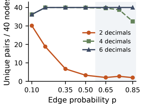
(c) RWSE feature diversity
