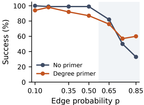
(a) 4B: degree lookup
