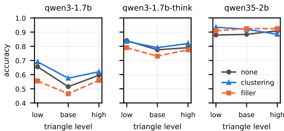
Figure 7: Rewiring: node_degree accuracy by triangle level (200 graphs per level; degree sequence and prompt length fixed; mean clustering 0.01, 0.31, 0.73).
