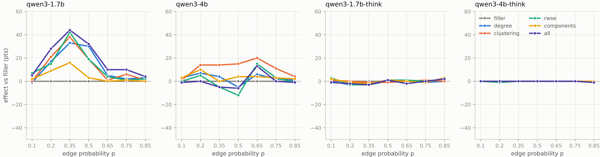
edge_existence - primer effect against a length-matched control, p = 0.1 to 0.85
