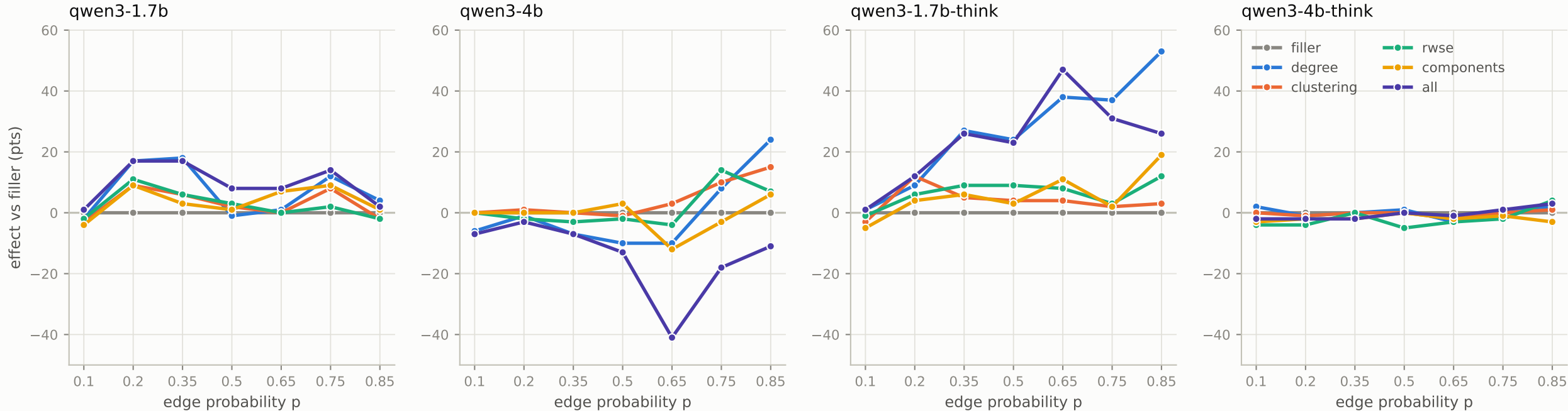
node_degree - primer effect against a length-matched control, p = 0.1 to 0.85
