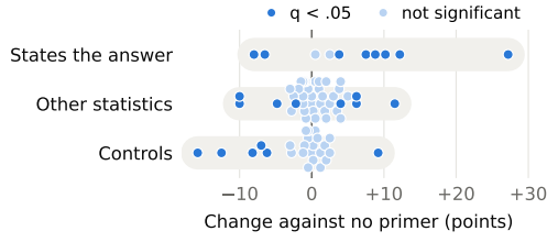
Figure 2: Primer effects grouped by what the primer states. Each dot is one cell of Table 1, the change in one arm’s accuracy on one task (points; right of zero is a gain; cells with at least 15% truncation omitted). Rows: states the answer (degree and all on node degree and edge count), other statistics (every other primer–task pair) and controls (components and filler). Filled: BH q < .05 against no primer. The largest gains come from primers that state the answer; other statistics move accuracy both ways, about as widely as the controls, and every significant filler effect is a loss.
