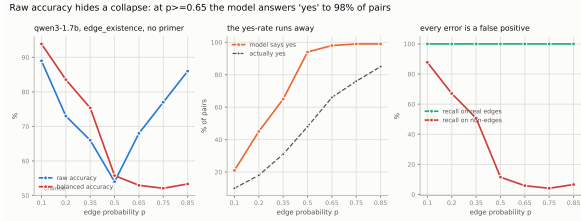
Figure 2: edge_existence under none, qwen3-1.7b. Accuracy falls to 54% at p=.50 and then rises again to 86% at p=.85 , which reads as a recovery. Balanced accuracy over the same responses does not recover: it reaches chance at p=.65 and stays there, because the model answers “yes” to 98–99% of pairs while 66–85% of them really are edges.
