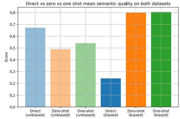
Fig. 5: Direct, zero-shot and one-shot mean semantic quality comparison for both datasets for the qwen3-14b model.
