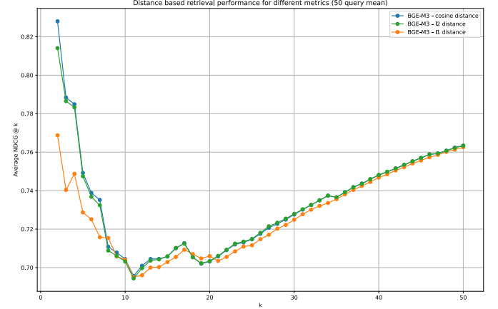
Fig. 5: Comparison of distance metrics using LLM-based NDCG@ k evaluation.
