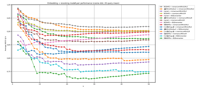
Fig. 6: LLM-based NDCG@ k evaluation of embedding model and reranker combinations.
