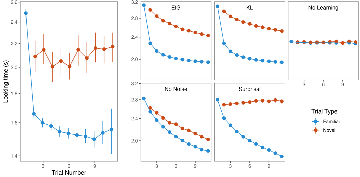
Figure 5: (fig:adult_exp1_res)Experiment 1, adult results
