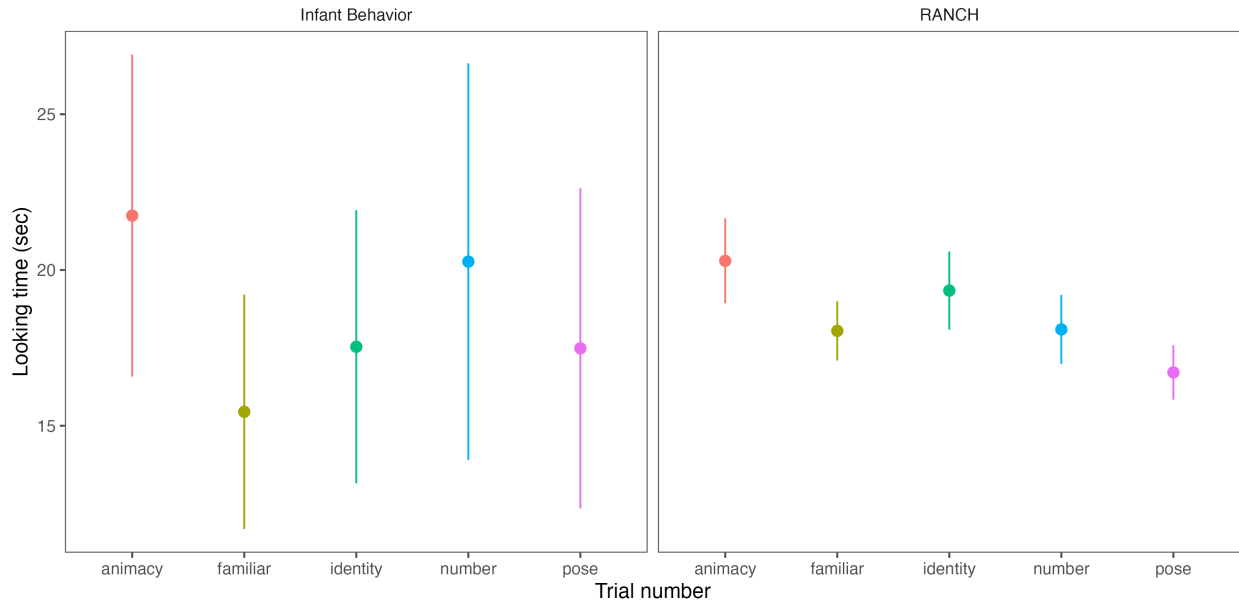
Figure 6: (#fig:infant_exp2_res)Experiment 2, infant results, combined across Zoom and Children Helping Science
