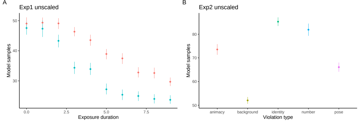
Figure 10: (#fig:wrong_scaling)The effect of scaling on model results. A) Experiment 1 with unscaled embeddings results in a reversal of background vs. deviant. B) Experiment 2 with unscaled embeddings results in an unintuitive ordering.
