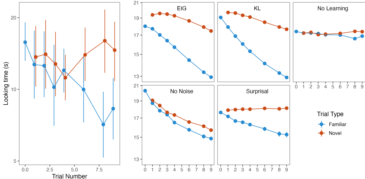
Figure 4: (#fig:infant_exp1_res)Experiment 1, infant results
