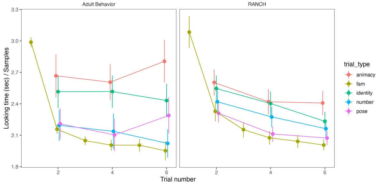
Figure 7: (#fig:adult_exp2_res)Experiment 2, adult results
