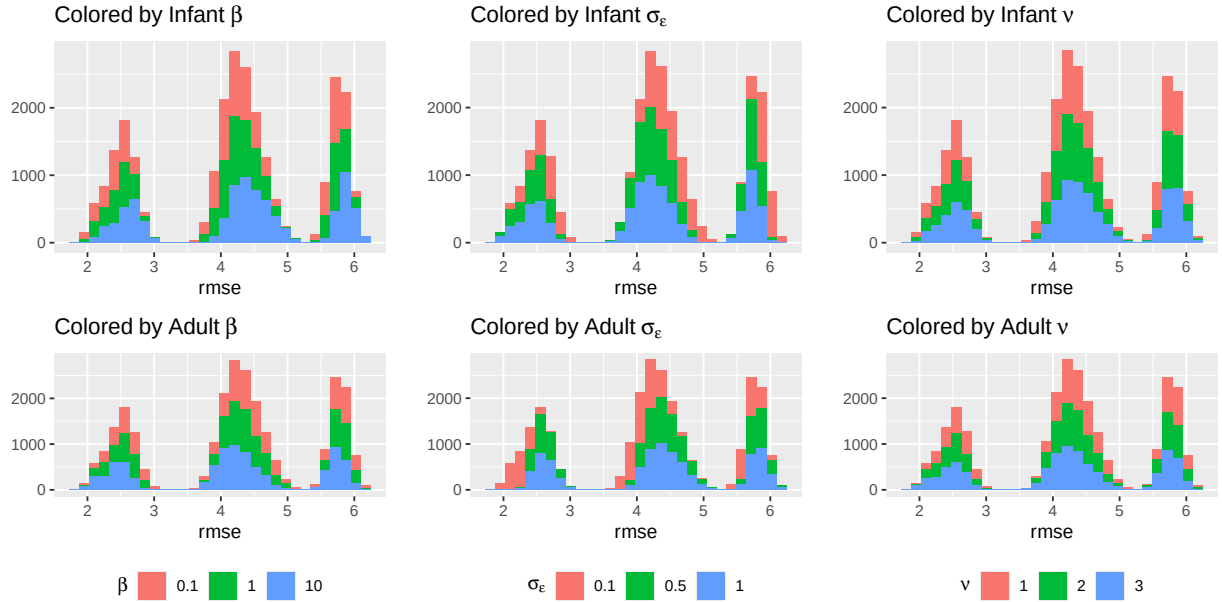
Figure 11: (#fig:parameter_interpretation)Histograms of model fit colored by priors. Results suggest that when the learner’s noise is high, RANCH fits infant data better.
