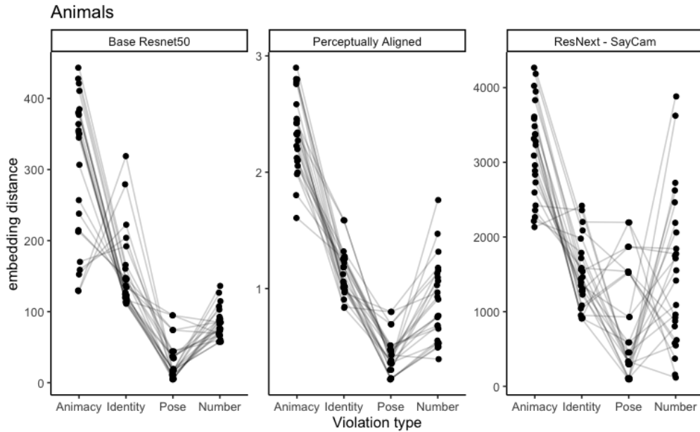
Figure 12: (#fig:embedding_distances)Embedding distances of different violation types for 1) a base ResNet50 model, 2) a perceptually aligned embedding model (Lee, 2022) and 3) a ResNet50 model trained on SAYCAM data (Orhan et al., 2020)
