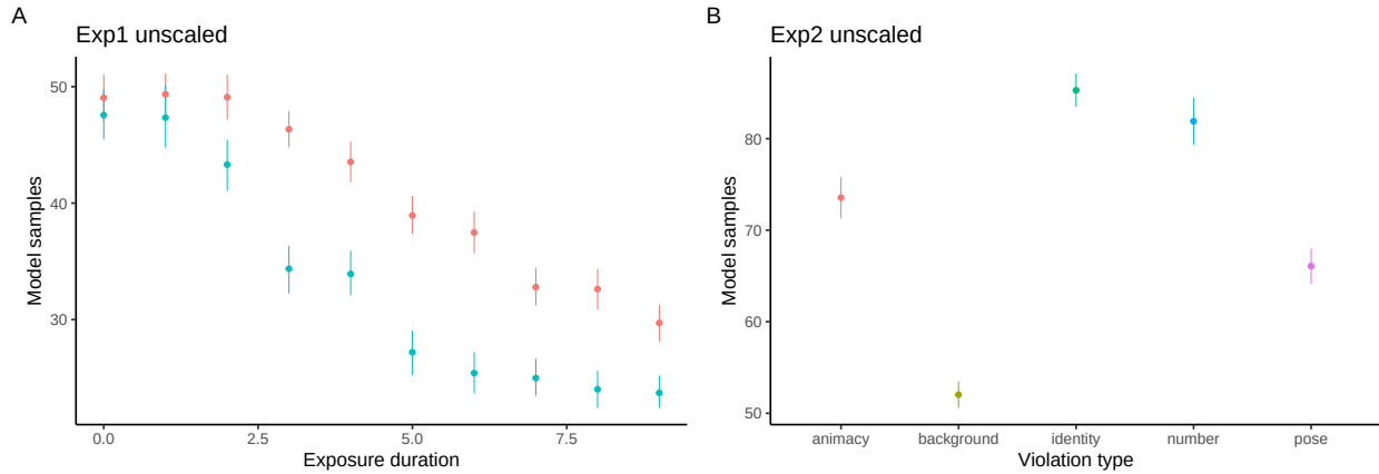
Figure 4: (#fig:wrong_scaling)The effect of scaling on model results. A) Experiment 1 with unscaled embeddings results in a reversal of background vs. deviant. B) Experiment 2 with unscaled embeddings results in an unintuitive ordering.
