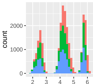
Colored by Adult \sigma_\epsilon
