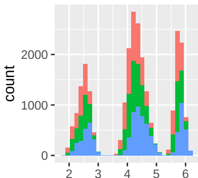
Colored by Adult \beta
