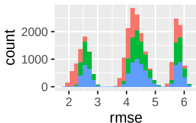
Colored by Adult \sigma_\epsilon
