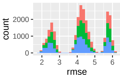
Colored by Adult \beta
