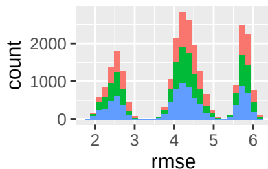
Colored by Adult v
