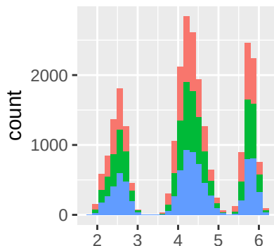
Colored by Adult v
