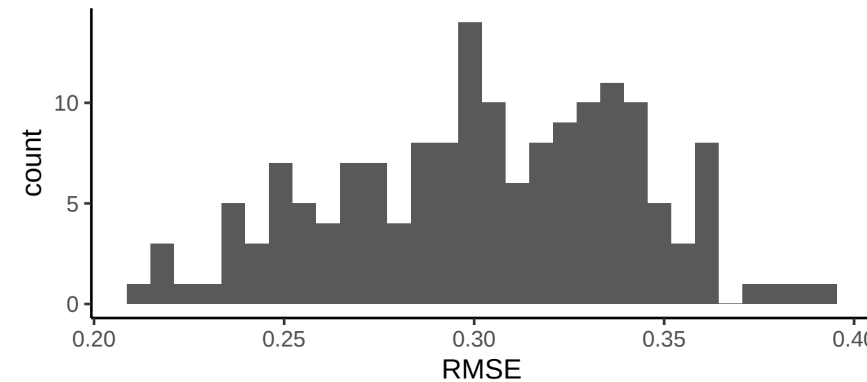
Surprisal
