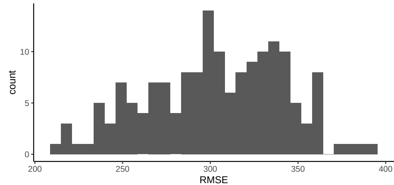
Surprisal
