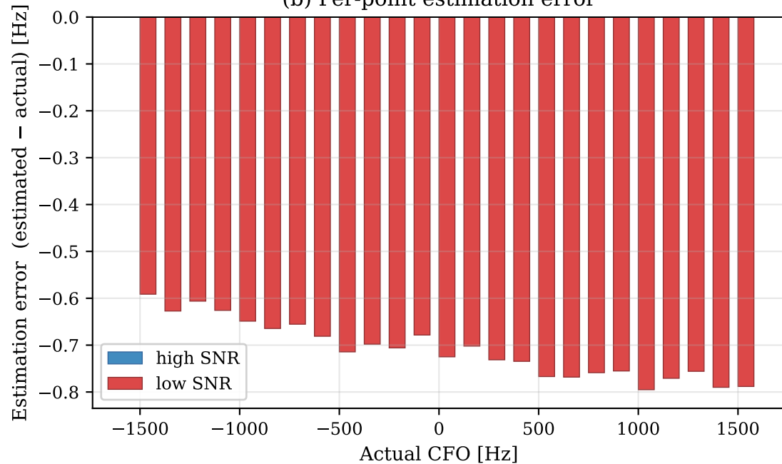
(b) Per-point estimation error
