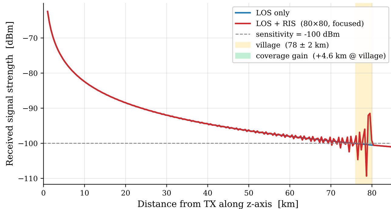
(a) RSSI vs distance
