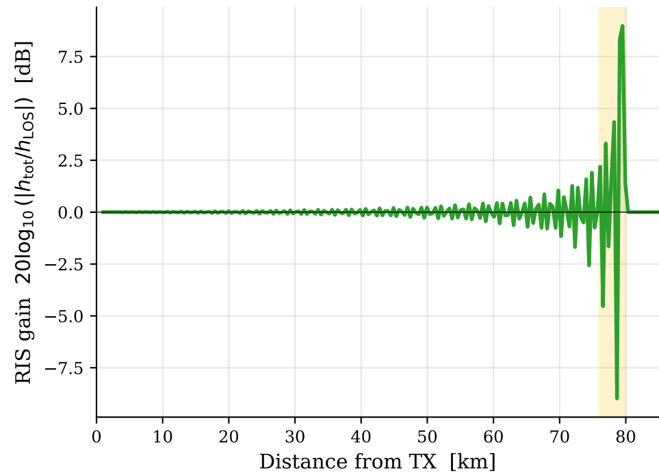
(b) RIS contribution vs distance
