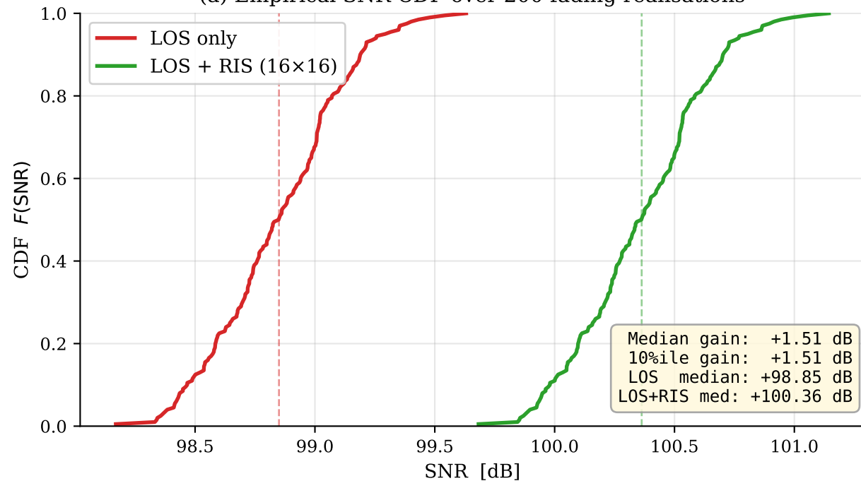
(a) Empirical SNR CDF over 200 fading realisations
