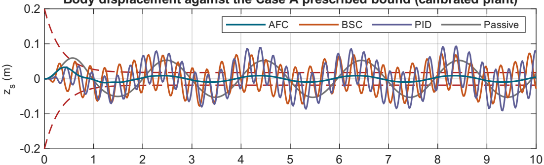
Body displacement against the Case A prescribed bound (calibrated plant)
