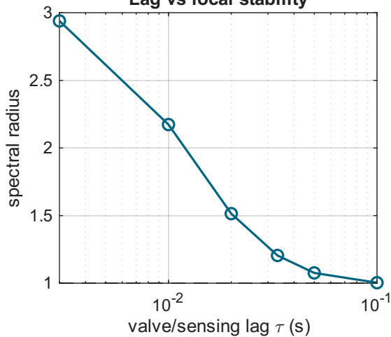
Lag vs local stability
