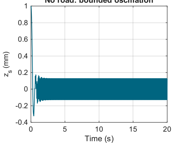
No road: bounded oscillation
