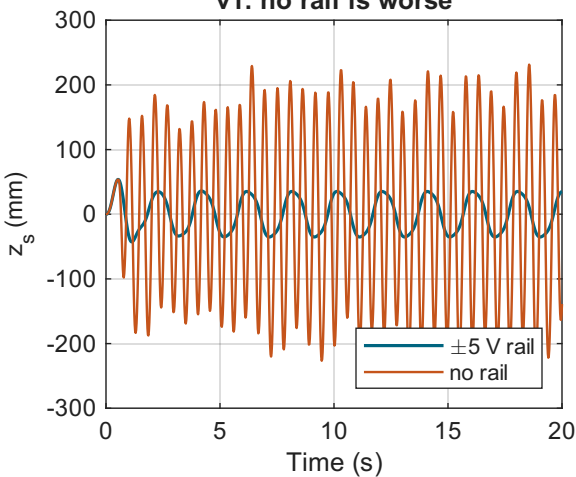
v1: no rail is worse
